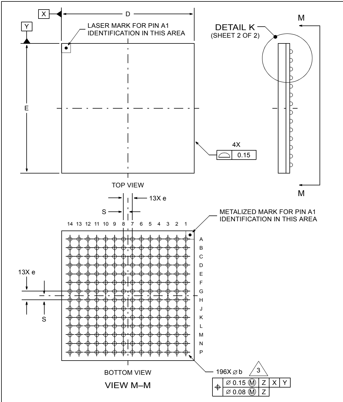
Figure 8-1. 196 MAPBGA Nomenclature
